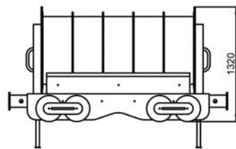
811020 Togvogn, tank HPL L2550xB1350xH1320 mm
